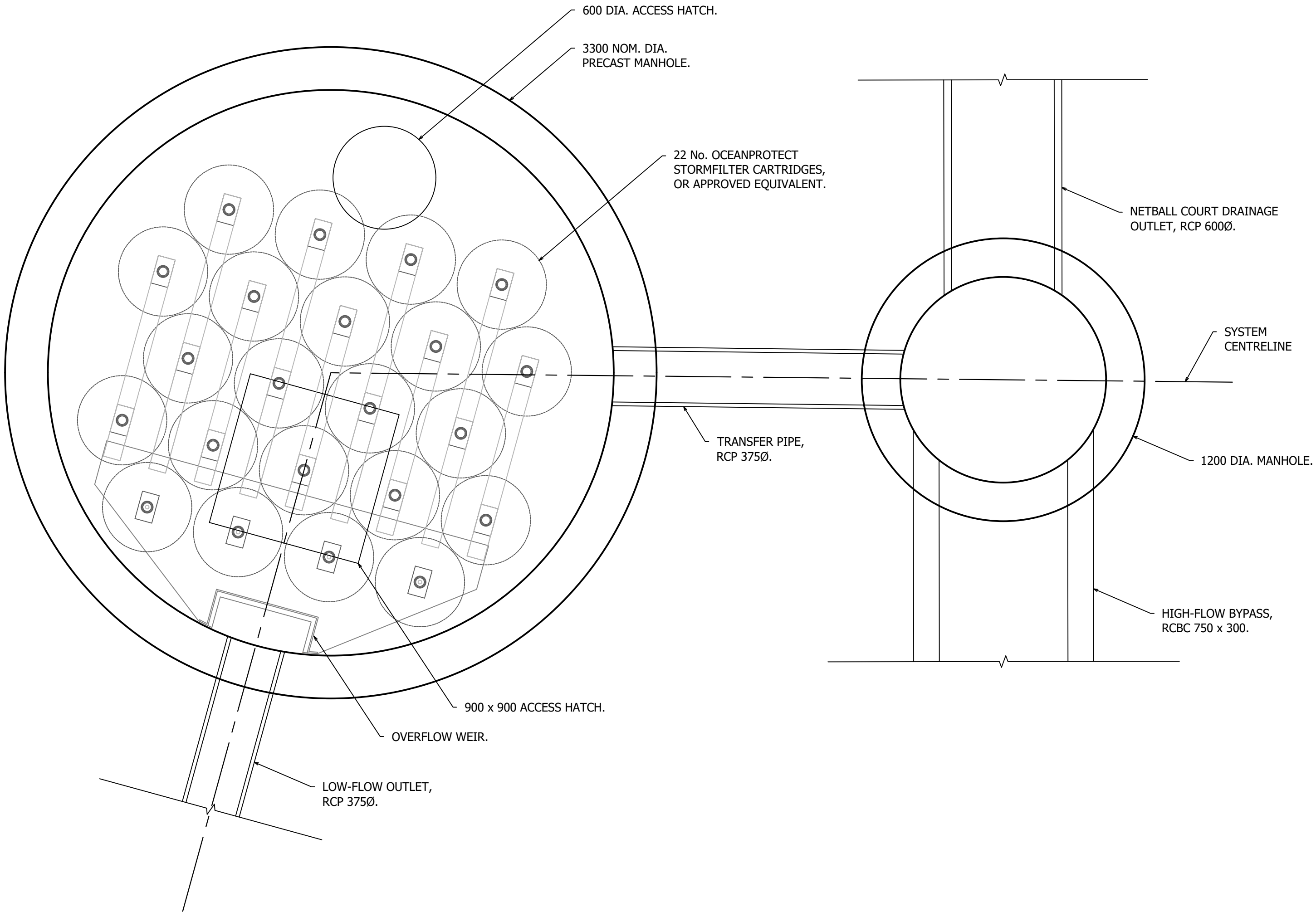
WSUD FILTRATION SYSTEM PLAN DETAIL SCALE 1:20
